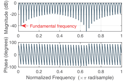
Fig. 11. Response of adaptive comb notch filter.
