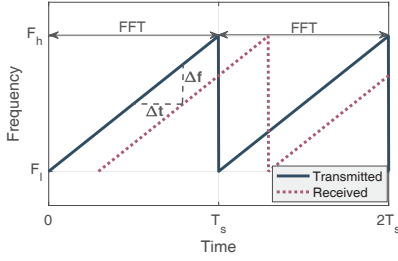
Fig. 3. FMCW sonar processing.
